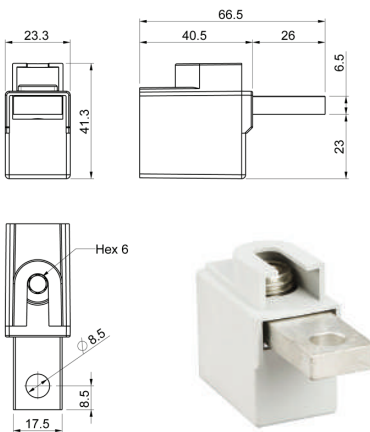
KKL 1x120T
