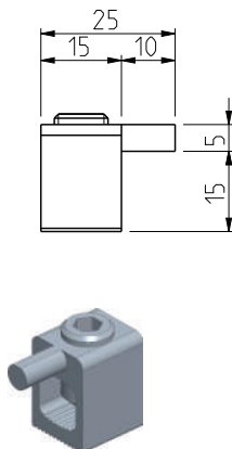
KKL 1x50
