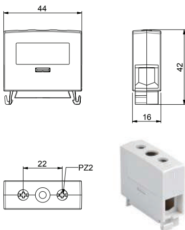
KC 1x35
