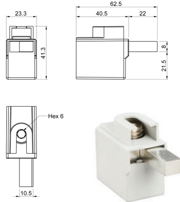
KKL 1x120T
