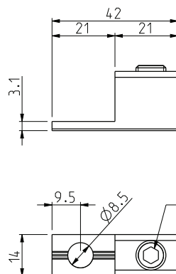
KKL 1x50
