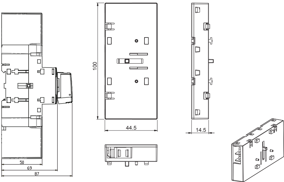
Auxiliary contact
