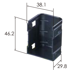
F Lever Cover Assy (6911-4401)
