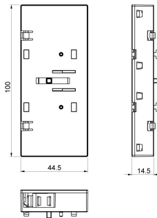
Auxiliary contact
