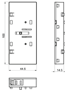
Auxiliary contact
