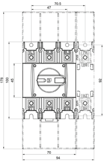
3 and 4 poles
