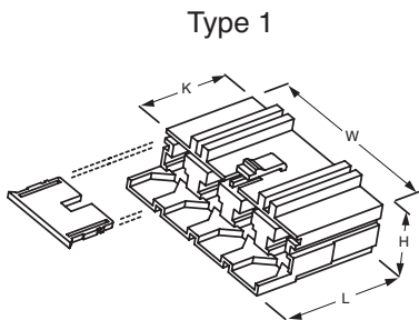
4 way housing for 8 mm receptacle (with secondary locking)
