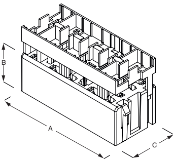
20 way socket for 2.8 mm mini fuses 10 fuses housing
