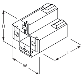
4 way relay housing
