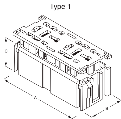
18 way / 2 relays housing
