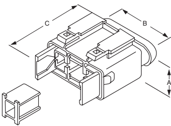
Housing for 8 mm Receptacle (with secondary locking)
