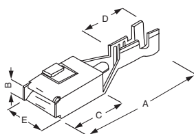
Micro-relay receptacles
