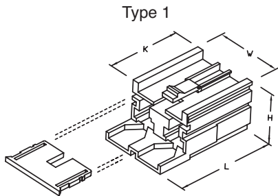
2 way housing for 8 mm receptacle (with secondary locking)
