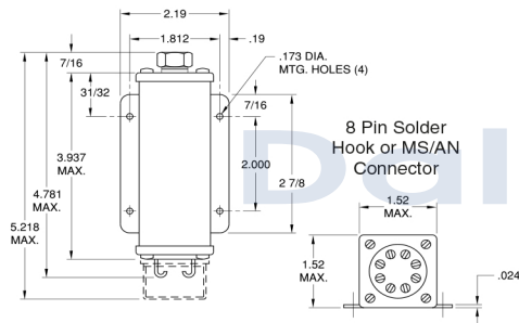
Panel Mount -H1, -H3
