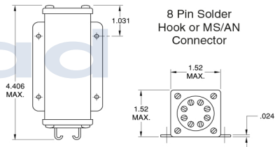
Panel Mount -9
