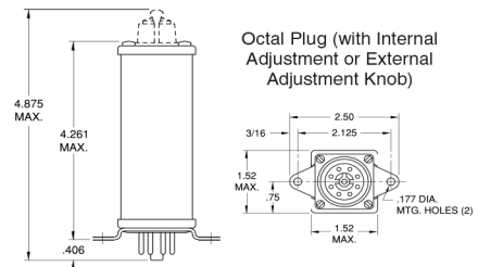
Chassis Mount -4, -5
