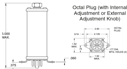
Chassis Mount -H2
