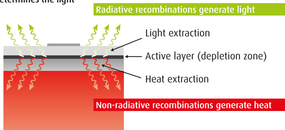
LEDs light and heat extraction
