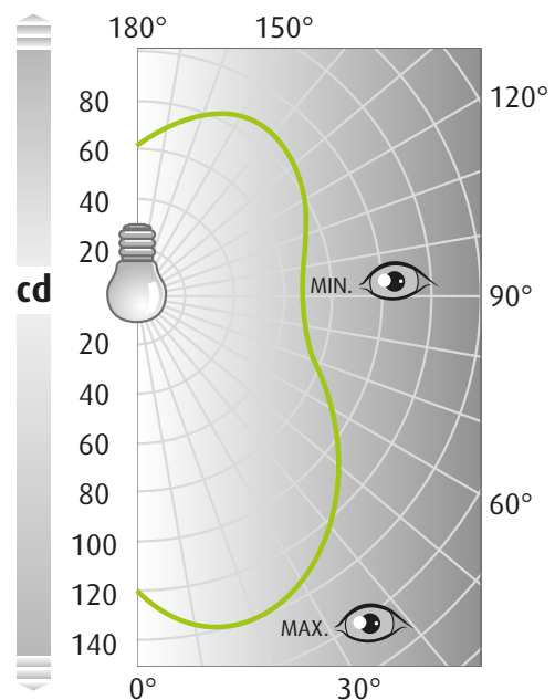
Intensity versus angular viewing
