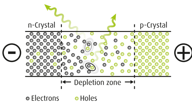
LEDs internal recombinations
