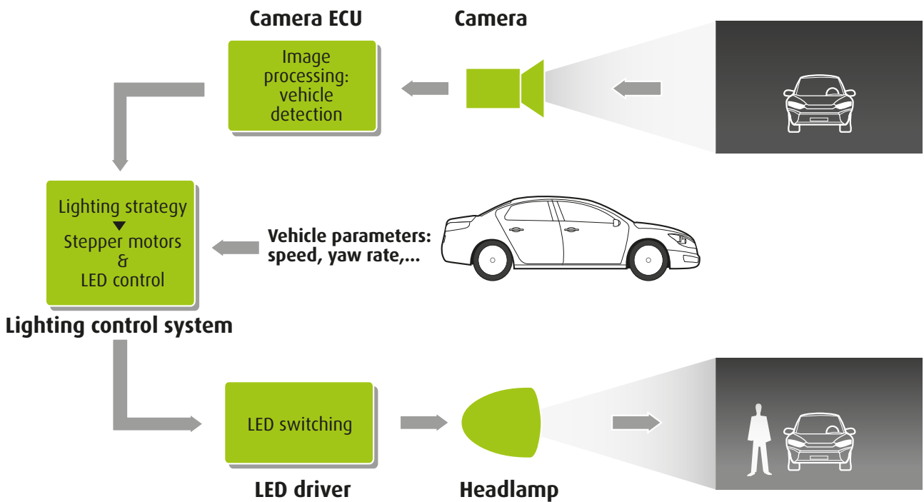
ADB bloc diagram
