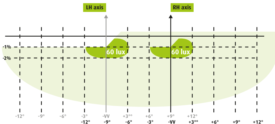
“classic” class C modes – H/V aiming
