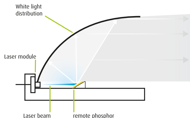
The blue laser light is converted to white light on the phosphor surface
