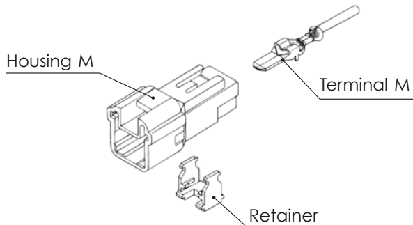
Connector M
