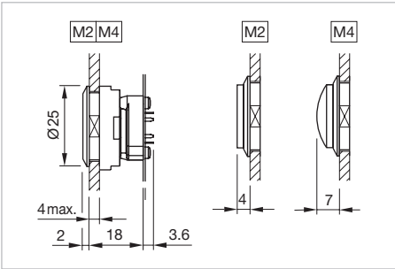
Dimensions [mm] M2 = Lens raised above bezel, M4 = Lens convex raised above bezel
