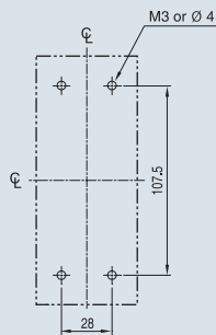
Panel drilling
