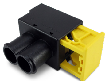
RECEPTACLE HOUSING (1355328-1)
