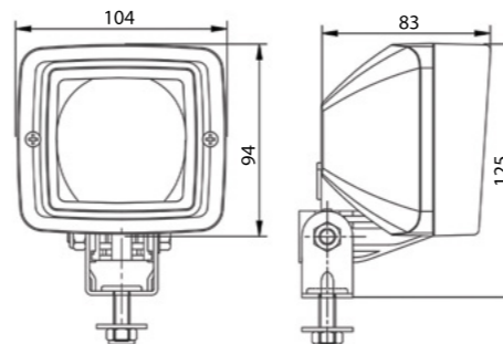
Dimension unit in mm
